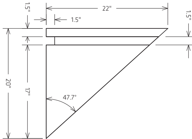
End View of Supports
