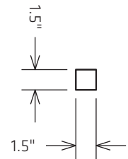
End View of Supports
